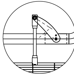
ACTIVATION DEVICE DETAIL
