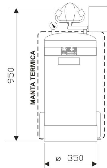
Ref. 6051-R2D2AC LAVAOJOS PORTATIL (50 Lts) Dimensiones en mm
