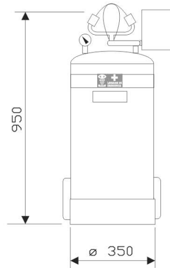
Ref. 6051-R2D2 LAVAOJOS PORTATIL (50 Lts) Dimensiones en mm
